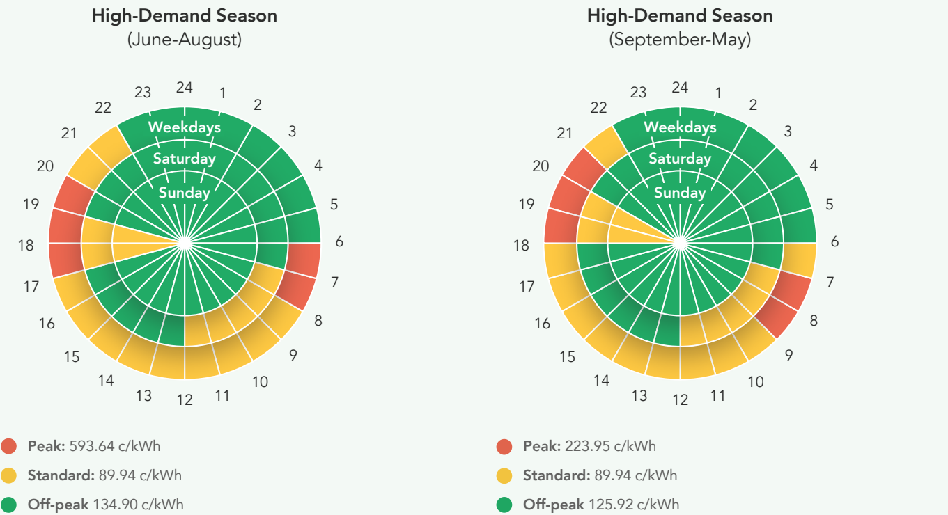
Figure 5: Eskom Wholesale Electricity Pricing System tariffs and time-of-use structure. Numbers around the graphics indicate the time of day. Source: Eskom Tariffs and Charges 2025-2026
