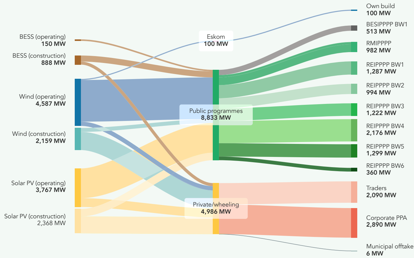
Figure 1: Large-scale RE adoption in South Africa at the end of March 2026
